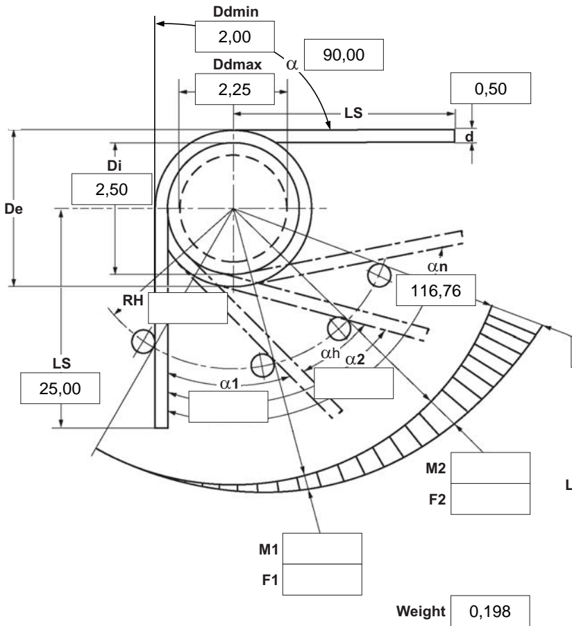
Spring test acc. to DIN ISO 2859/1 test level II
