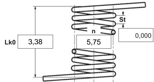
Spring test acc. to DIN ISO 2859/1 test level II
